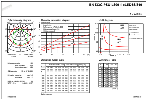
IFGU1_BN132CPSUL6001xLED6S840
