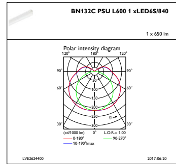
IFPC1_BN132CPSUL6001xLED6S840
