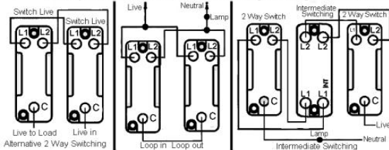
2 Way and Intermediate Switching Wiring Methods
